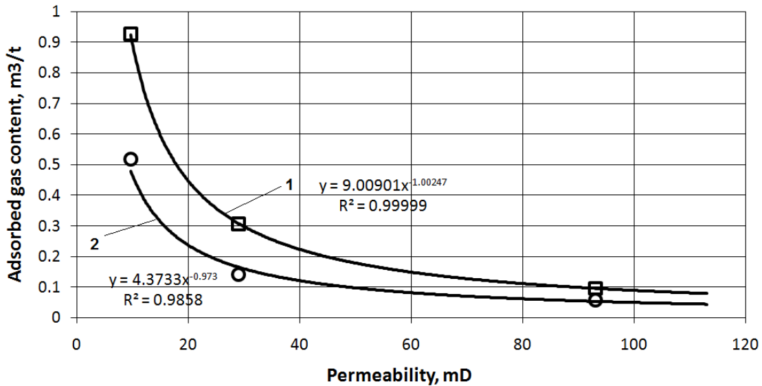
Figure 5 – Graphical dependences of adsorbed gas content from model permeability for different temperatures at the pressure 3 MPa
