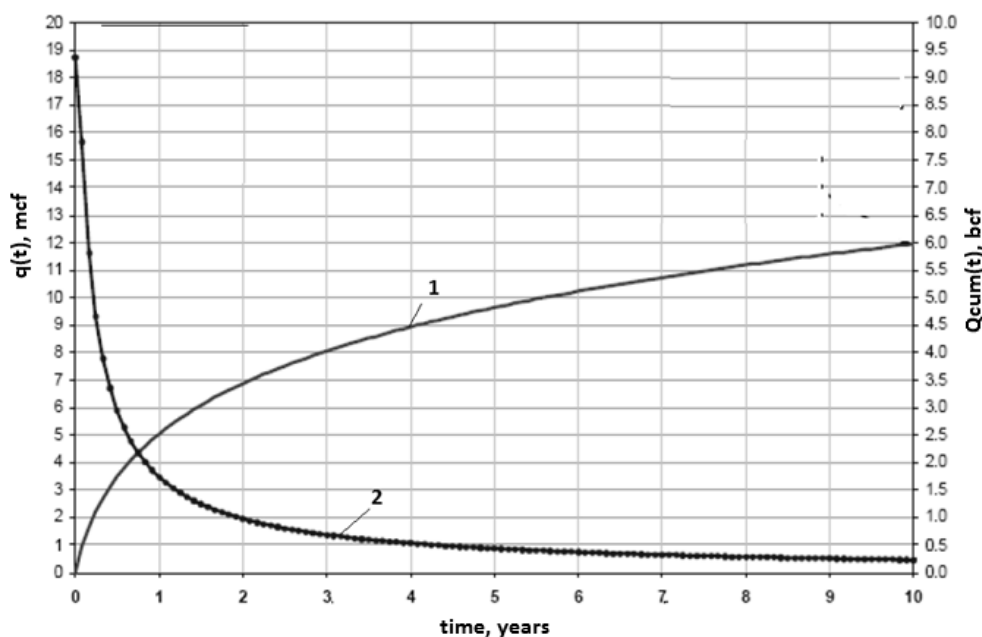
Figure 1 – Production decline curves for Heynesville shale
